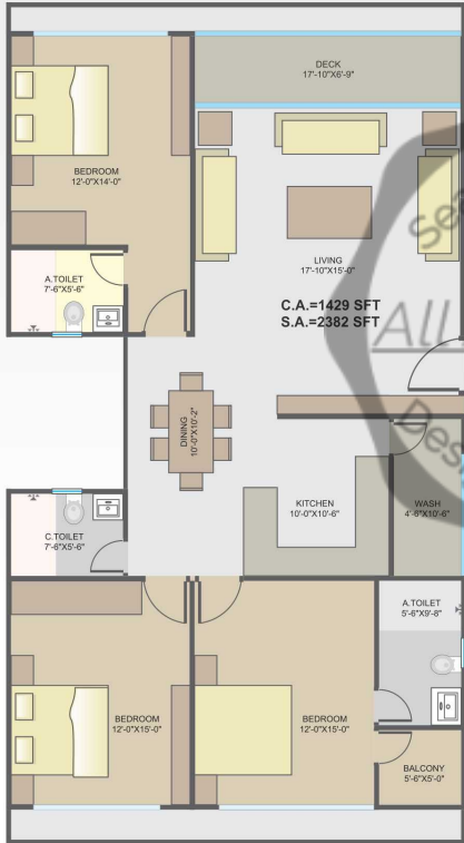
1st floor to 6th floor plan
